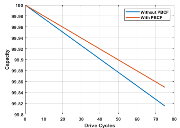
Fig. 8. Battery degradation abatement with PBCF
